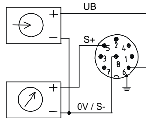
8-pin connector
