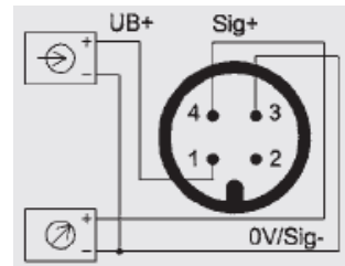
Circular connector M12x1.5
